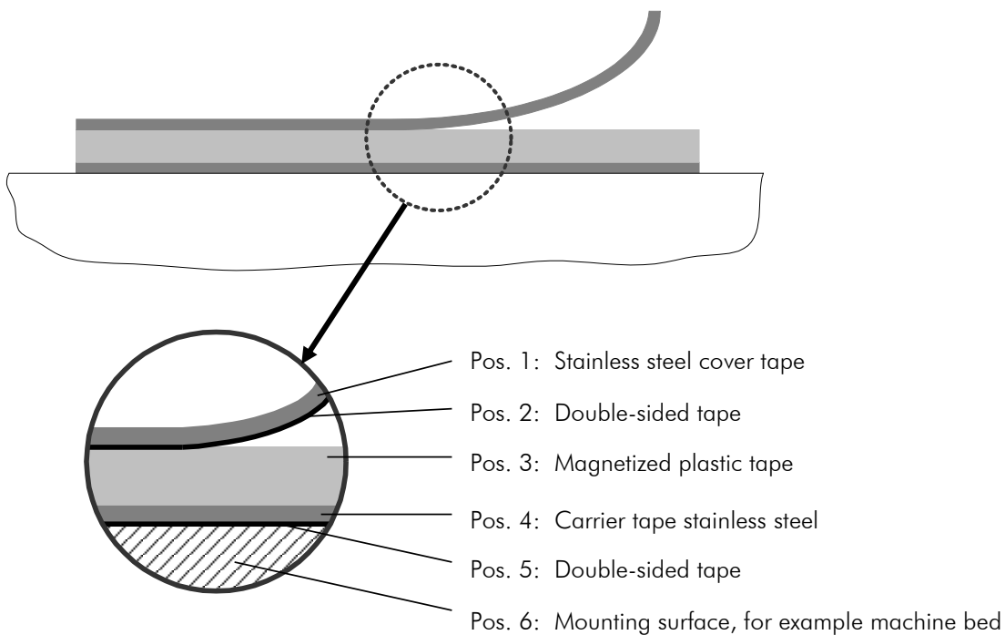
Figure 3: Components of the magnetic tape
