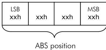
Figure 9: CAN interface
