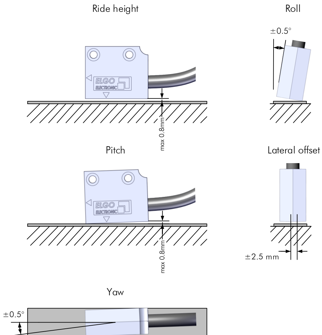
Figure 6: Tolerances
