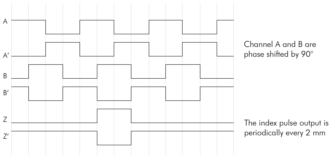
Figure 2: Pulse diagram
