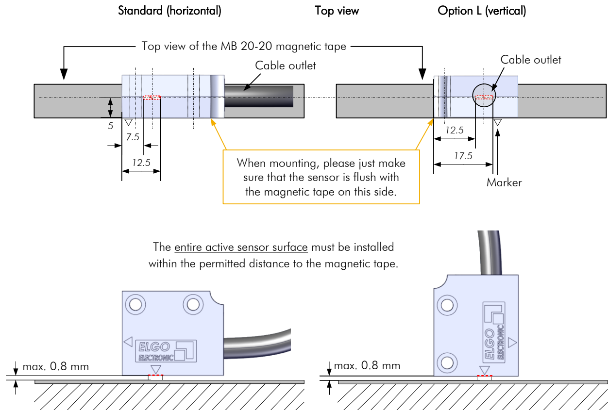
Figure 7: Alignment of the Sensor
