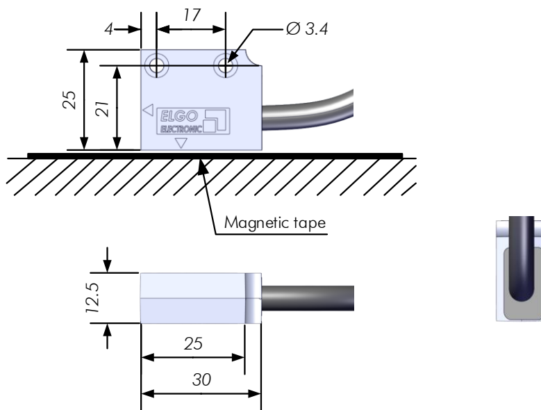
Figure 4: Dimensions Sensor
