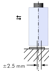
Offset (lateral)
