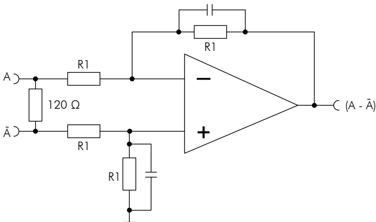
Figure 3: Example of a follow-up circuit
