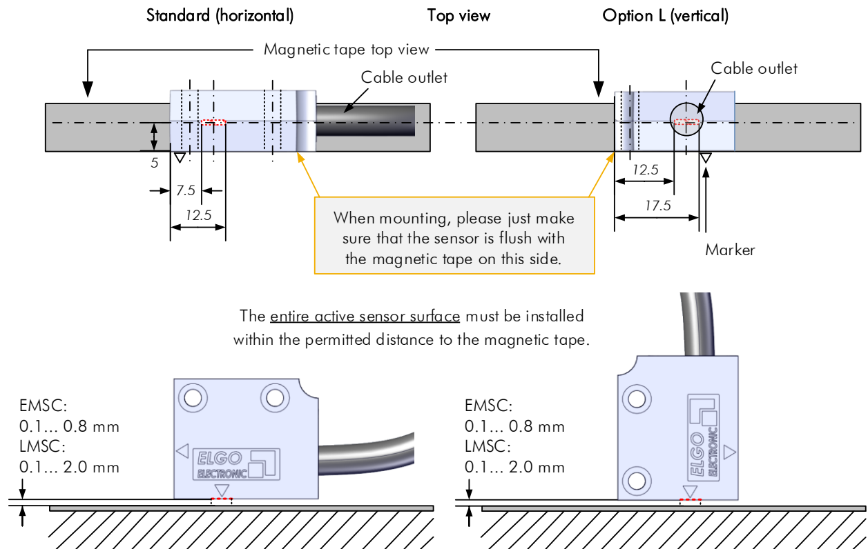
Figure 5: Alignment of the Sensor
