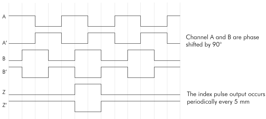
Figure 2: Pulse diagram
