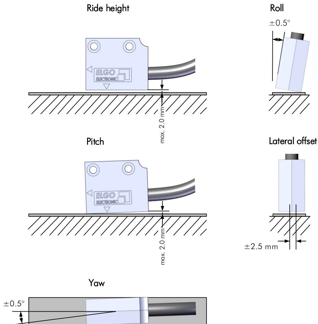
Figure 6: Tolerances
