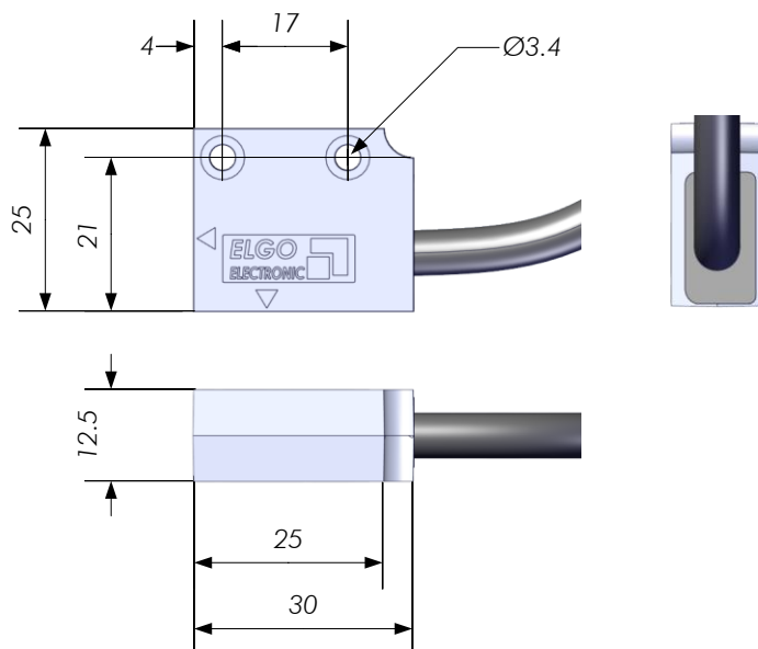
Figure 1: Dimensions housing
