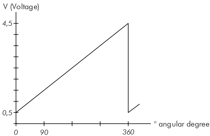
Figure 4: Output signal analog
