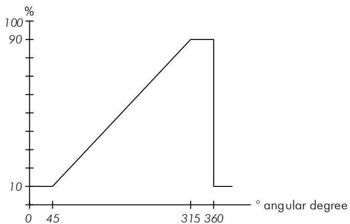
Figure 5: Output signal PWM
