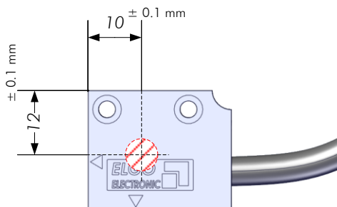
Figure 3: Alignment of the magnet to sensor
