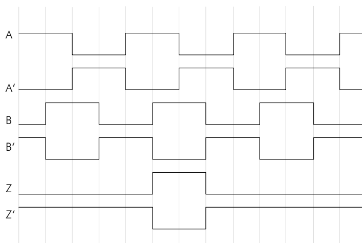
Figure 2: Pulse Diagram
