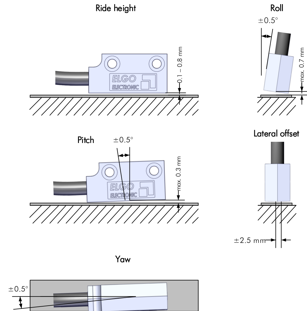
Figure 6: Sensor mounting tolerances
