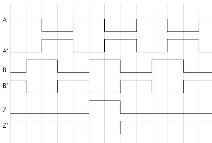
Figure 2: Pulse Diagram
