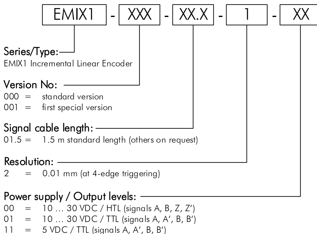
Figure 7: Type Designation
