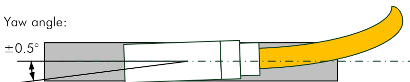
Figure 9: Mounting tolerances
