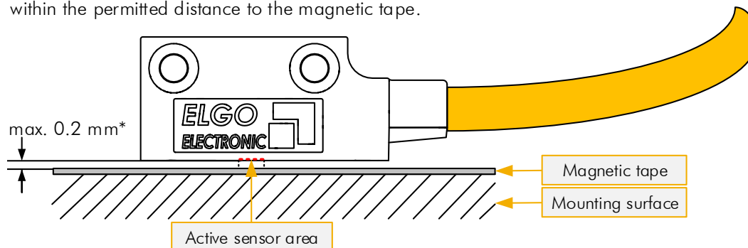
Figure 7: Reading Distance and Active sensor area
