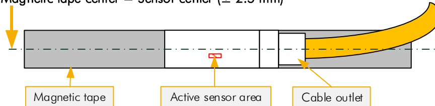
Figure 6: Sensor mounting and alignment
