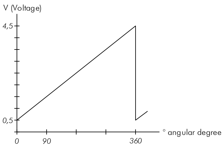
Figure 4: Signal level analog
