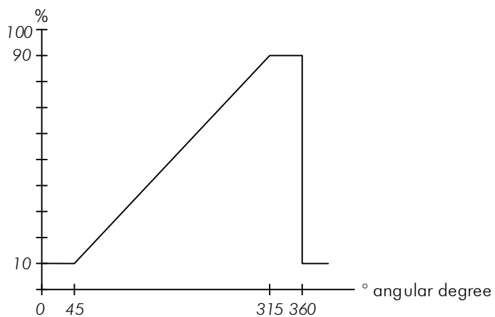
Figure 5: Signal level PWM
