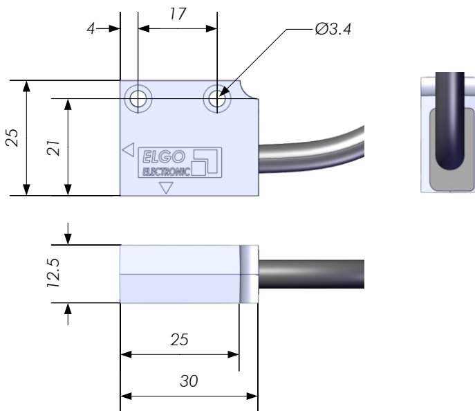
Figure 1: Dimensions housing
